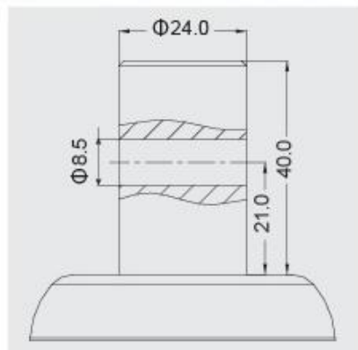
NO.04 \Phi 24 \times 40-\Phi 8.5
