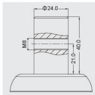
NO.03 \Phi 24 \times 40-M8
