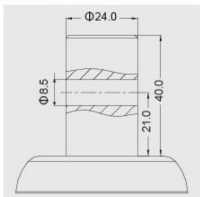
NO.04 \Phi 24 \times 40-\Phi 8.5
