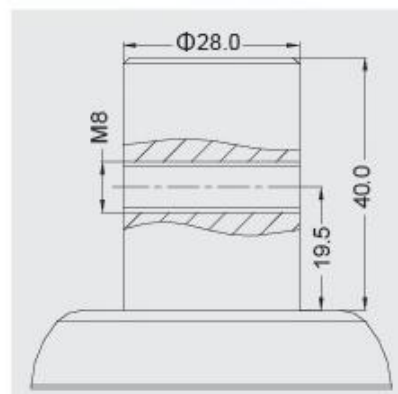
NO.06 \Phi 28 \times 40
