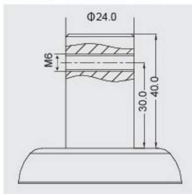
NO.02 \Phi 24 \times 40-M6
