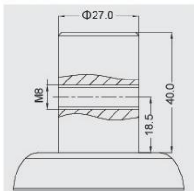
NO.05 \Phi 27 \times 40
