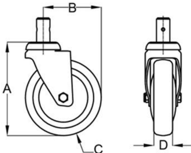
Dimensions(unit:mm) 5575-82G-8
