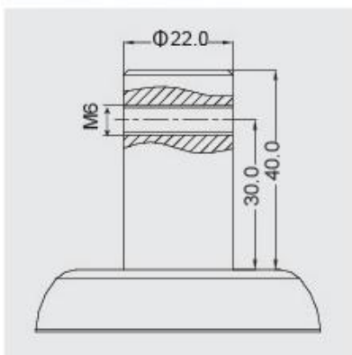
NO.01 \Phi 22 \times 40
